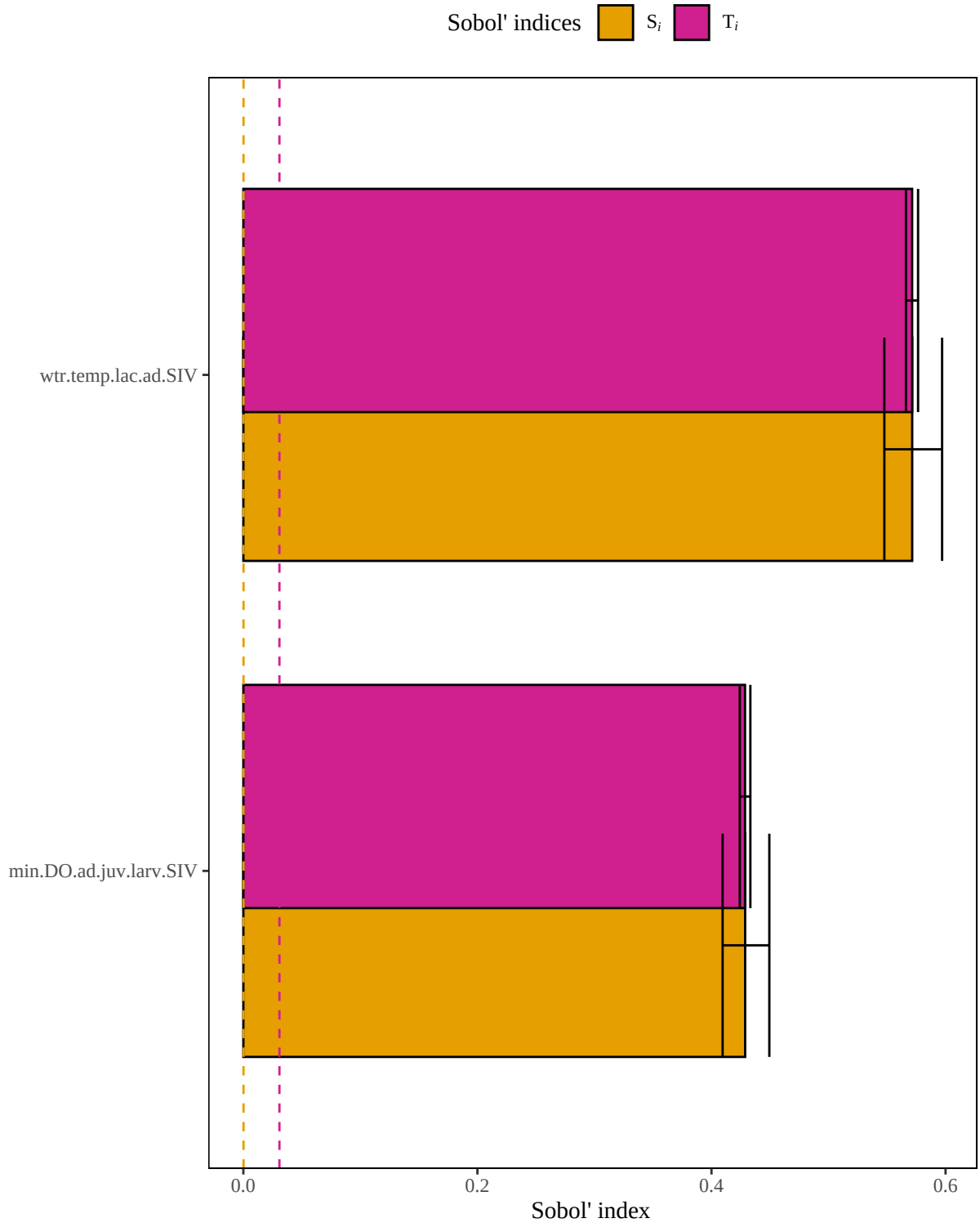
Figure 4. Results of a sensitivity analysis for the striped bass Inland Lac Ad model based on an arithmetic mean structure. Dashed lines represent baseline numerical approximation error for S_i and T_i ( i.e. , dummy variables).
