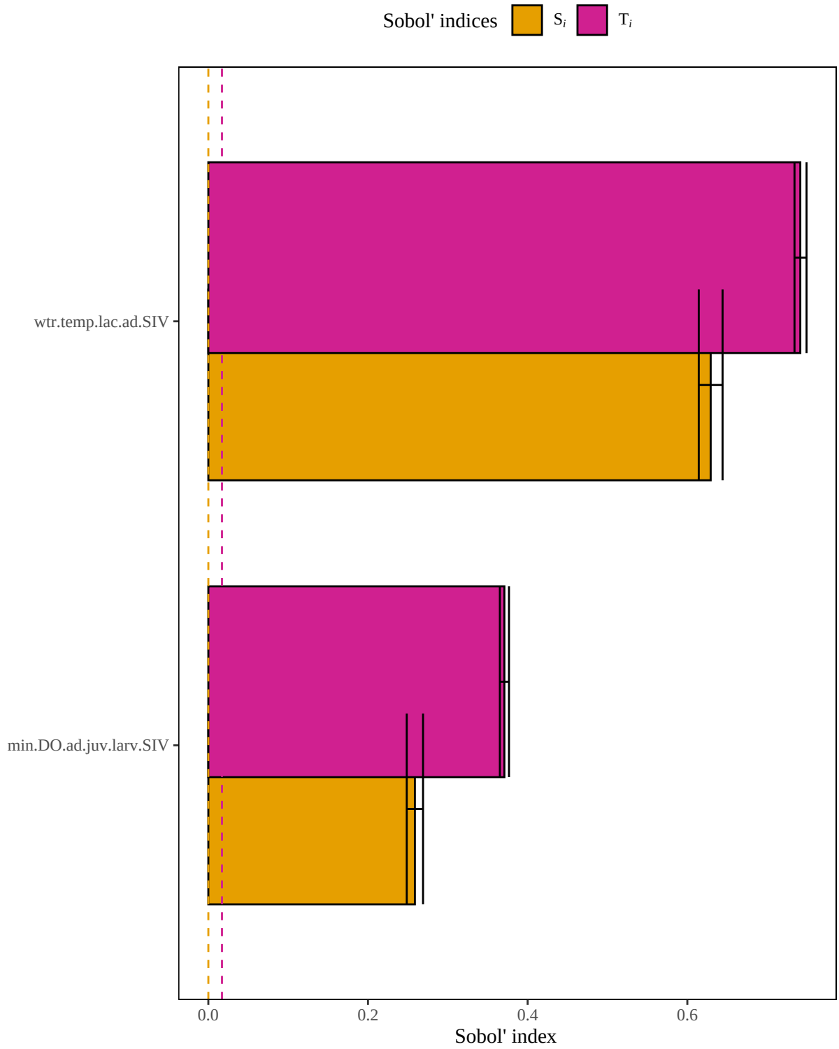
Figure 3. Results of a sensitivity analysis for the striped bass Inland LacAd model based on the original limiting factor model outlined in Crance (1984). Dashed lines represent baseline numerical approximation error for S_i and T_i ( i.e. , dummy variables).
